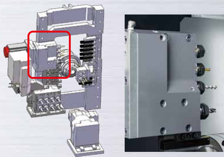
4-spindle cross live tools (Standard)
