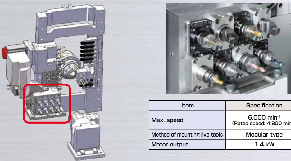
8-spindle back drive (Linear 6-axis machine) (Standard)
