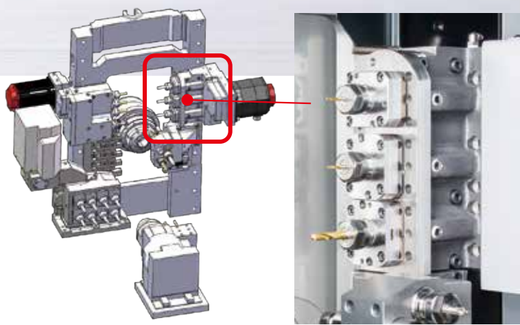
Rear drive (Option)
