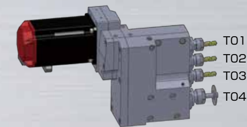
4-spindle cross live tools (Standard)
