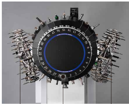
Left-side tool stoker Turret magazine Right-side tool stoker
